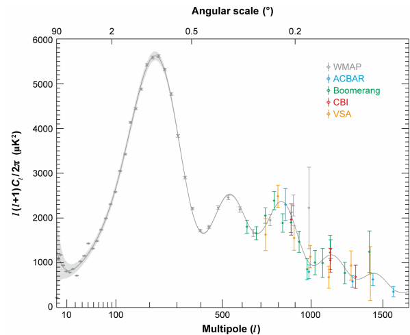
Figure 4: Observed angular power spectrum of CMB temperature anisotropies, plotted as \ell(\ell + 1)C_\ell/2\pi versus the multipole moment \ell . The factor \ell(\ell + 1)/2\pi approximately flattens the spectrum at large \ell , making the oscillatory structure more apparent. (Image credits [8])
