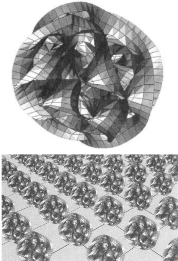
Figure 25: Calabi-Yau Manifold
