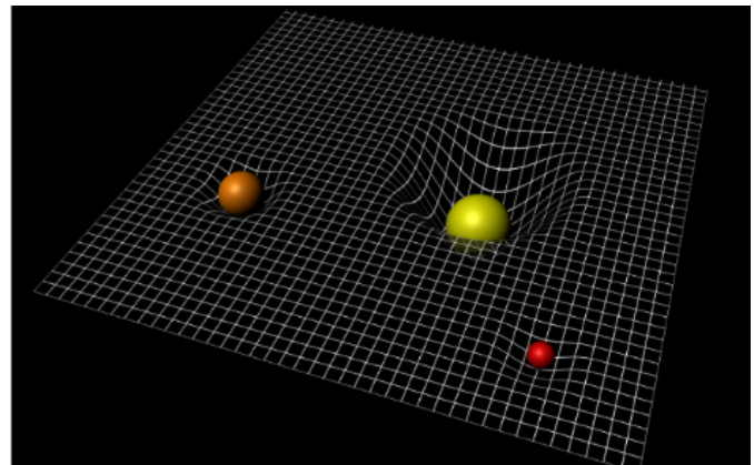
Figure 22: Warping of spacetime by a massive object
